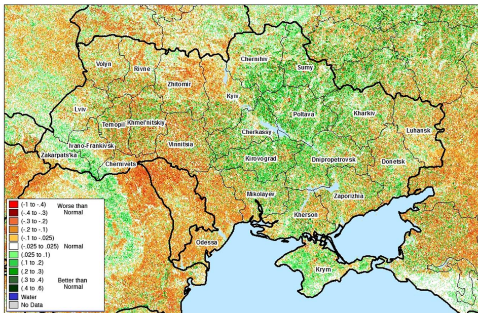
Ukraine: MODIS NDVI Anomaly Departure from Average August 5-12, 2015
